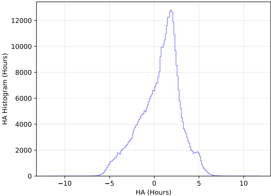
roll_pause_mjdp120_v3.4_10yrs All sky z band: HA Histogram
