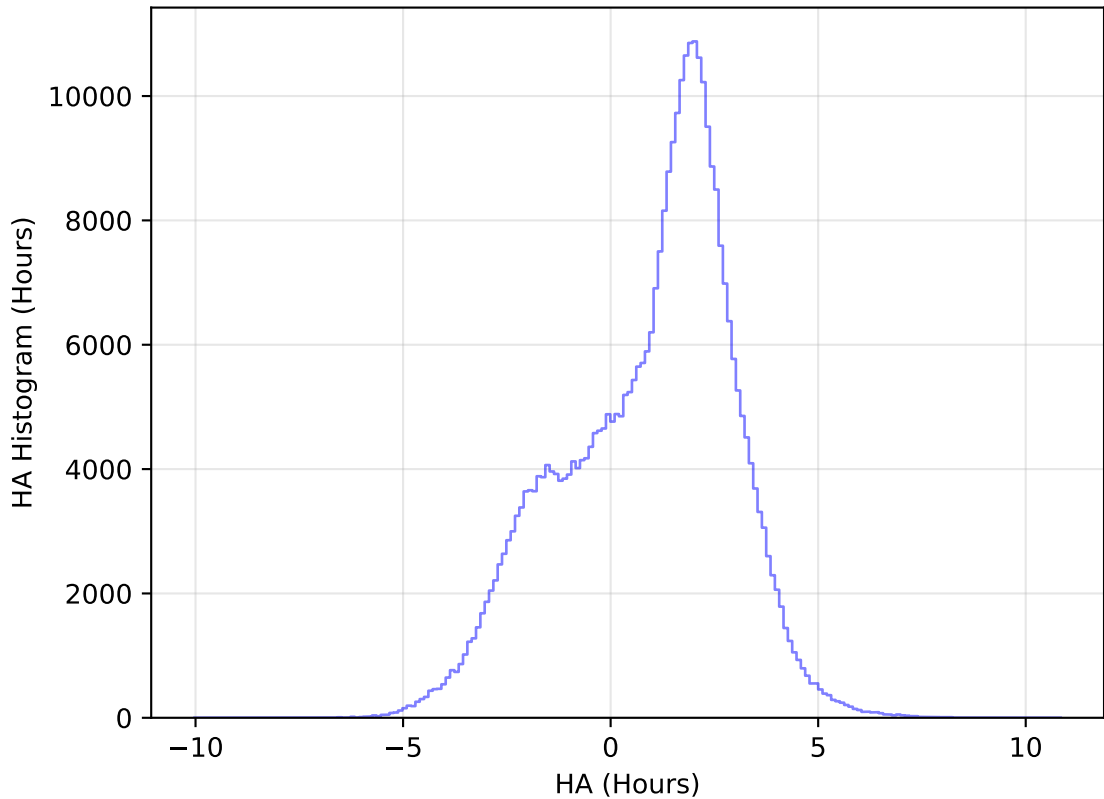
roll_pause_mjdp120_v3.4_10yrs All sky y band: HA Histogram
