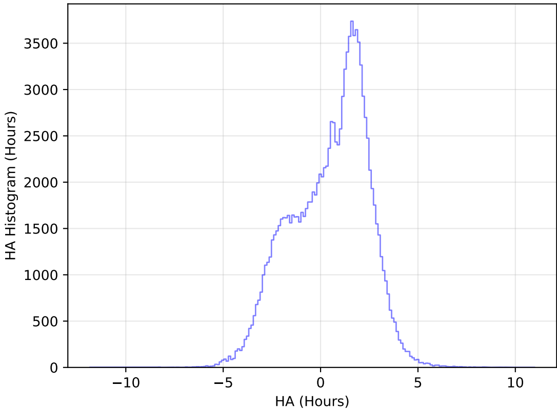
roll_pause_mjdp120_v3.4_10yrs All sky u band: HA Histogram
