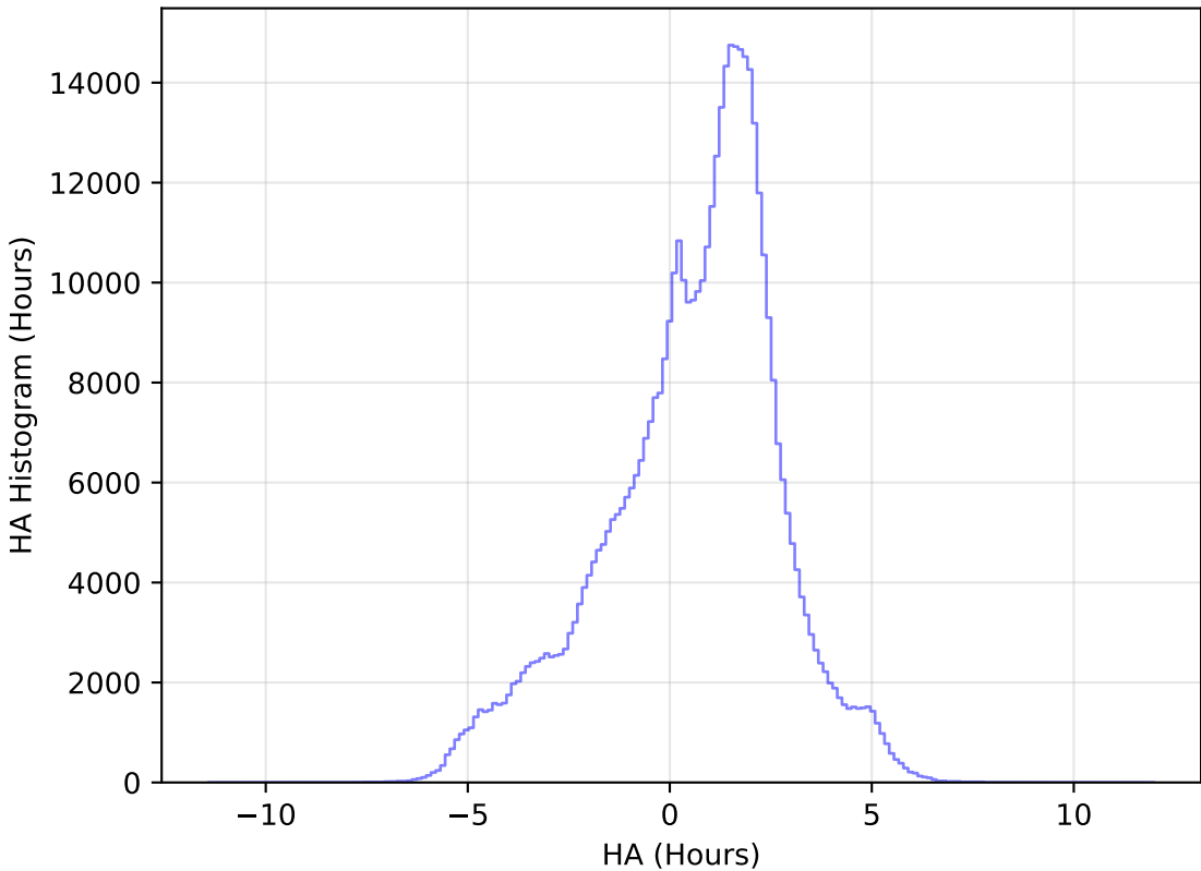
roll_pause_mjdp120_v3.4_10yrs All sky i band: HA Histogram
