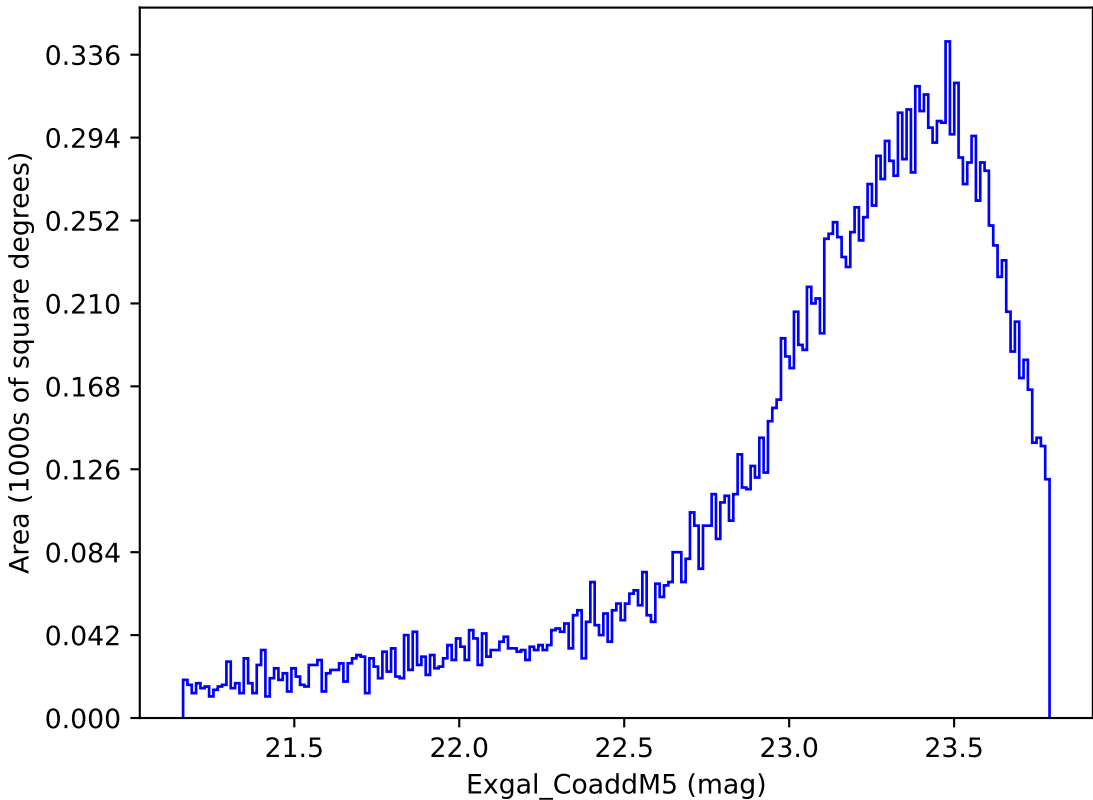
roll_pause_mjdp120_v3.4_10yrs Yr 3-4 y band: Exgal_CoaddM5
