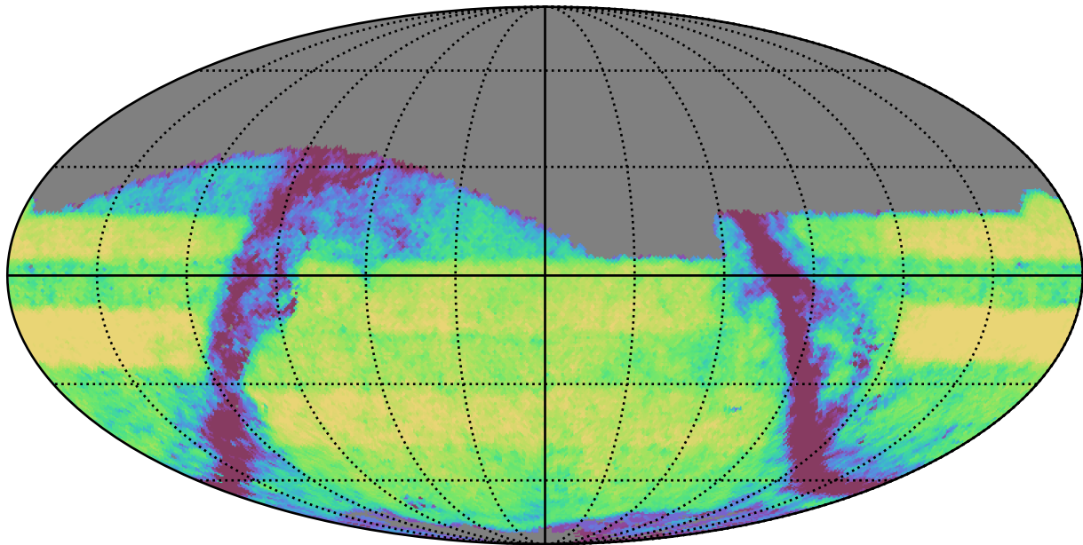
roll_pause_mjdp120_v3.4_10yrs Yr 3-4 i band: Exgal_CoaddM5
