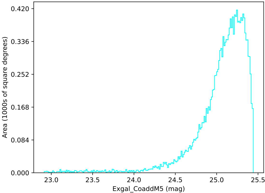
roll_pause_mjdp120_v3.4_10yrs WFD u band: Exgal_CoaddM5
