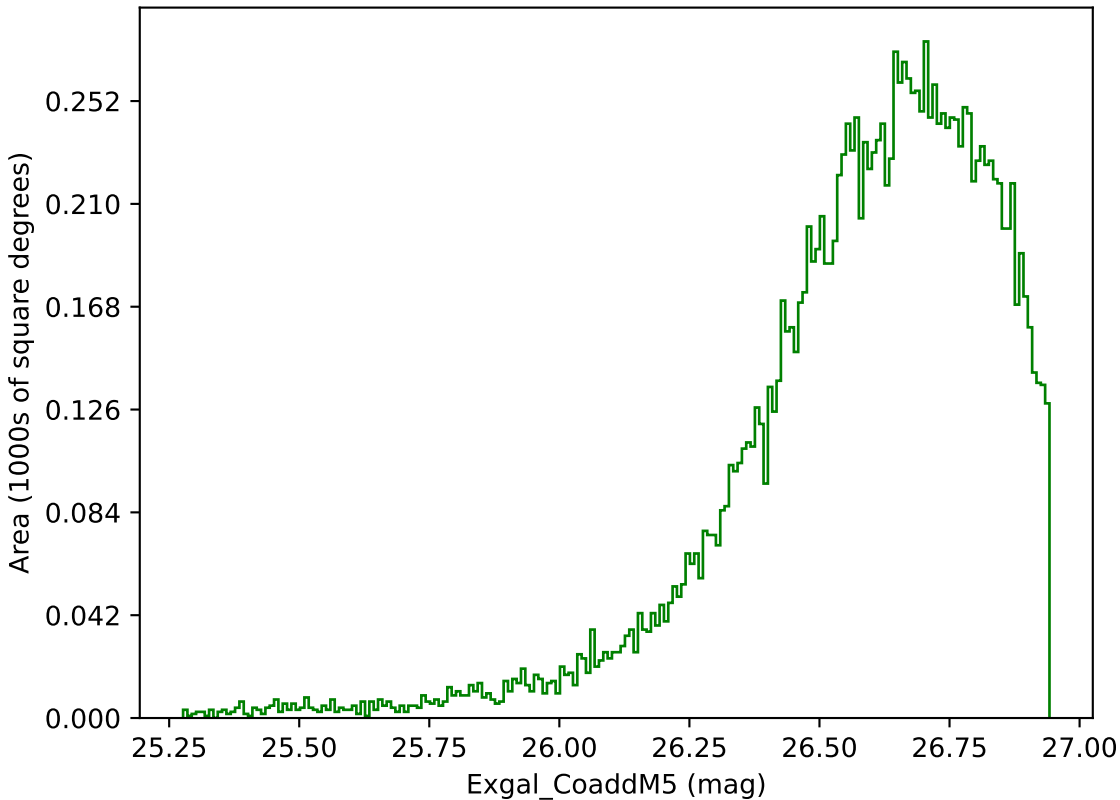
roll_pause_mjdp120_v3.4_10yrs WFD g band: Exgal_CoaddM5
