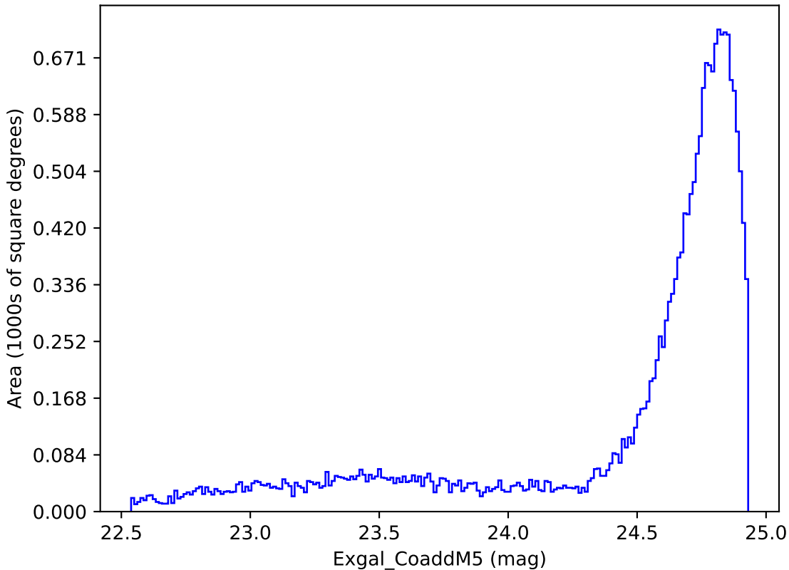
roll_pause_mjdp120_v3.4_10yrs All sky y band: Exgal_CoaddM5
