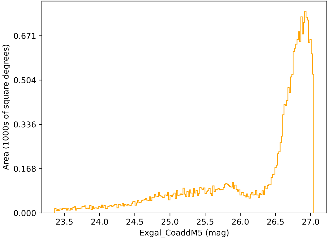
roll_pause_mjdp120_v3.4_10yrs All sky r band: Exgal_CoaddM5
