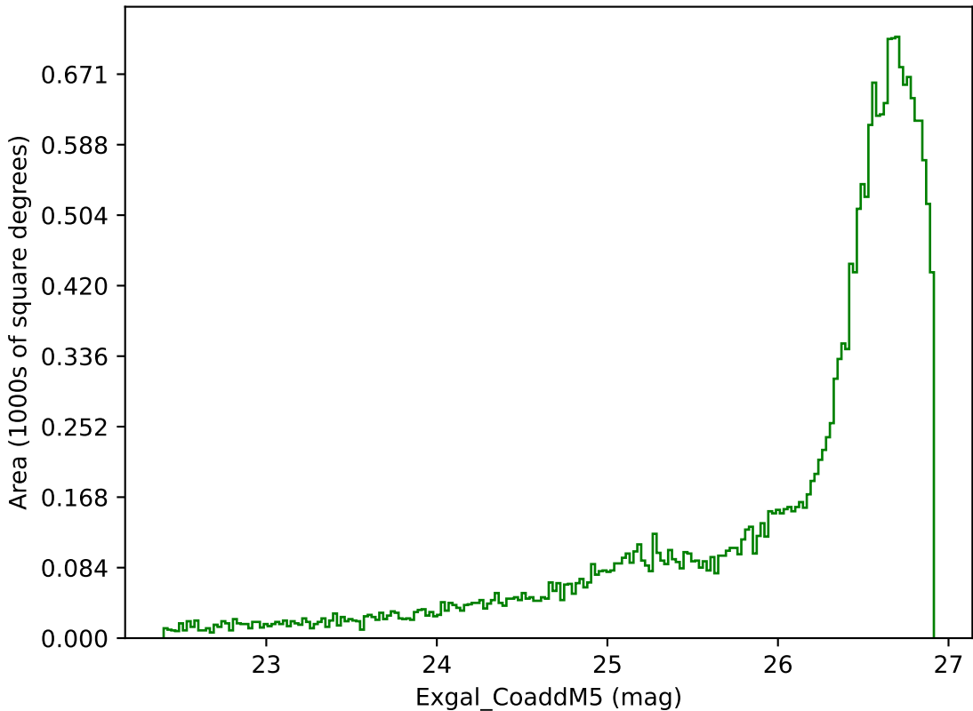
roll_pause_mjdp120_v3.4_10yrs All sky g band: Exgal_CoaddM5
