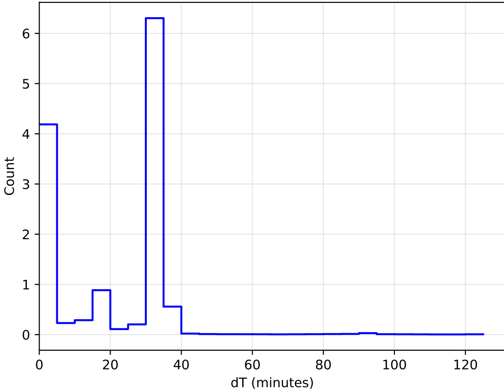
roll_pause_mjdp120_v3.4_10yrs All sky: DeltaT Histogram 1e6
