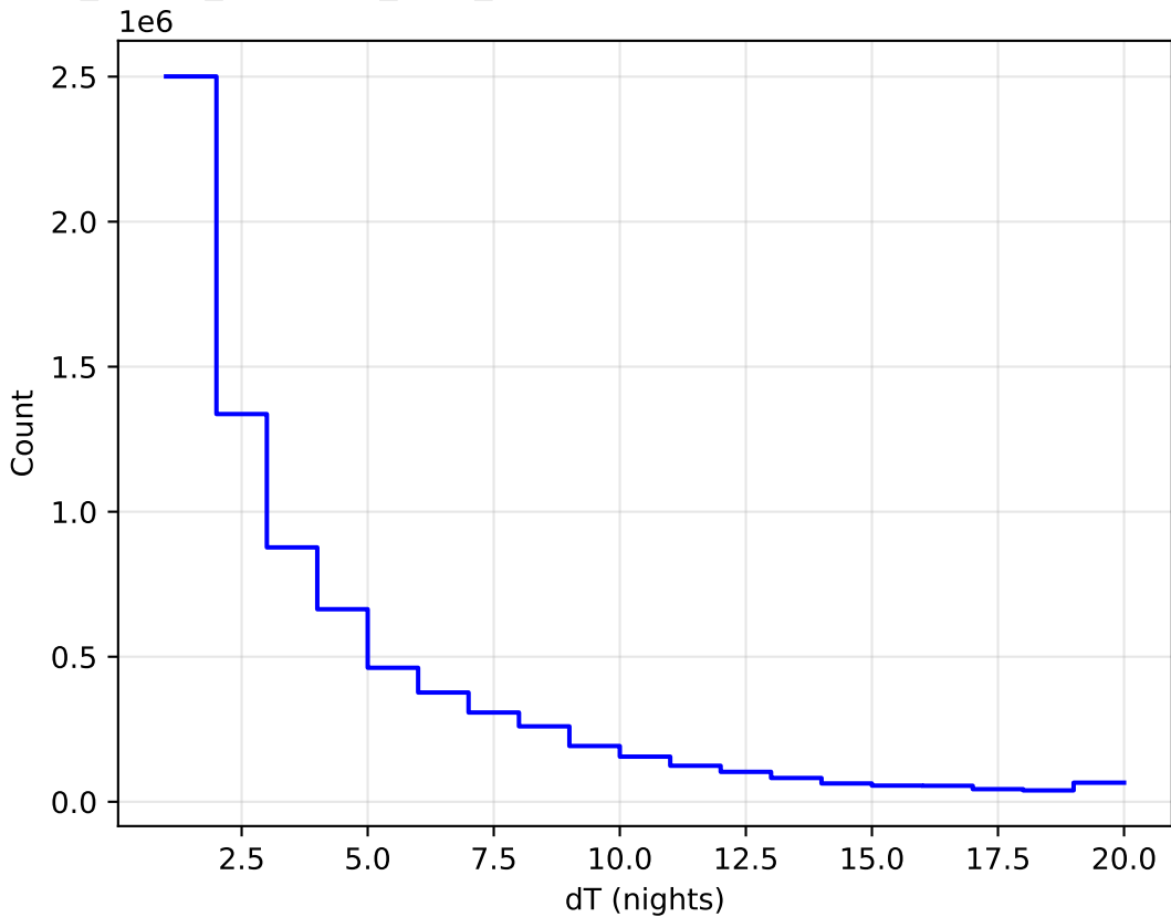
roll_pause_mjdp120_v3.4_10yrs WFD all bands: DeltaNight Histogram
