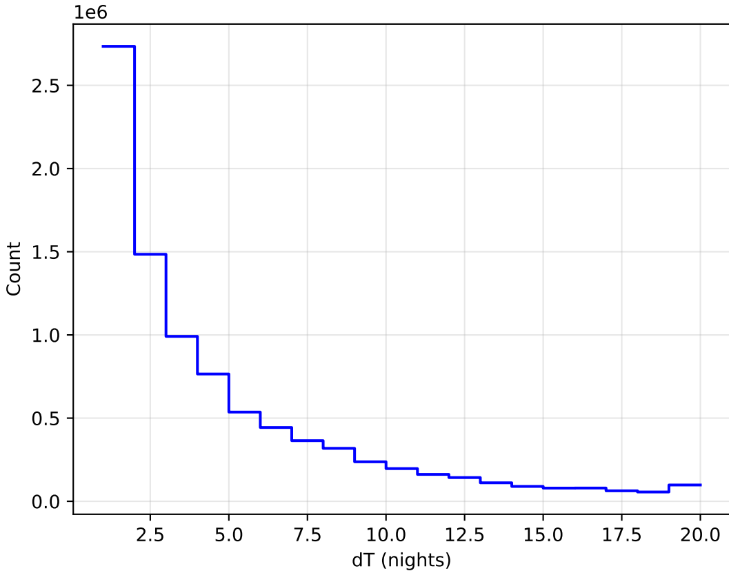
roll_pause_mjdp120_v3.4_10yrs All sky all bands: DeltaNight Histogram
