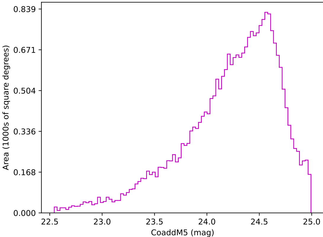
roll_pause_mjdp120_v3.4_10yrs Yr 3-4 z band: CoaddM5
