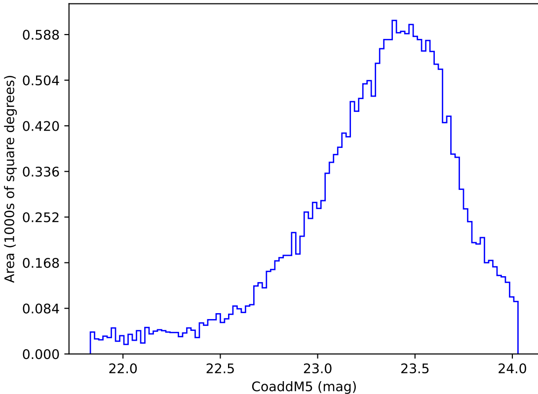
roll_pause_mjdp120_v3.4_10yrs Yr 3-4 y band: CoaddM5
