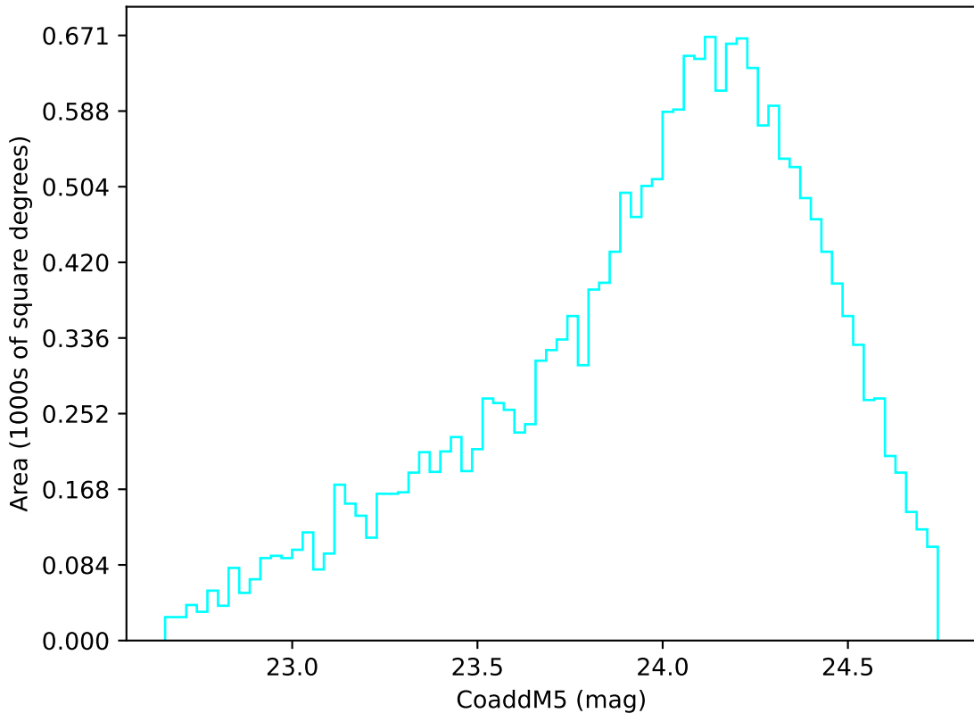
roll_pause_mjdp120_v3.4_10yrs Yr 3-4 u band: CoaddM5
