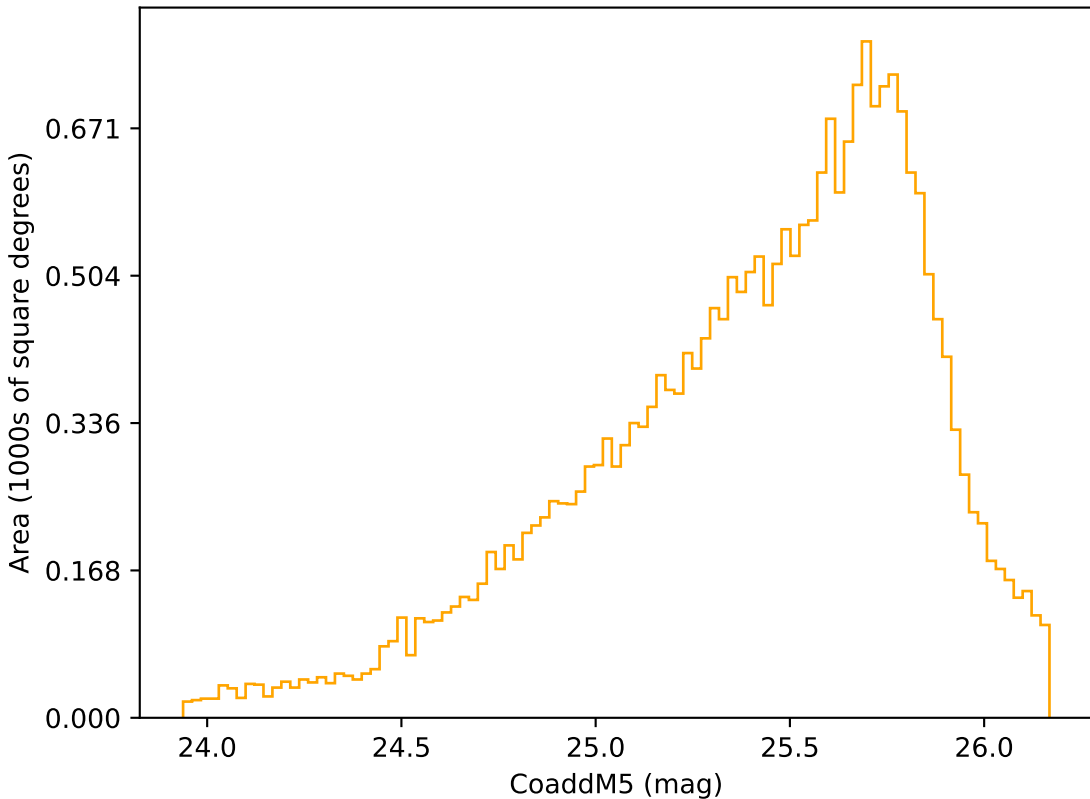
roll_pause_mjdp120_v3.4_10yrs Yr 3-4 r band: CoaddM5
