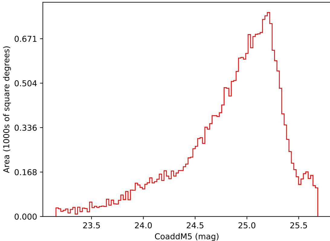
roll_pause_mjdp120_v3.4_10yrs Yr 3-4 i band: CoaddM5
