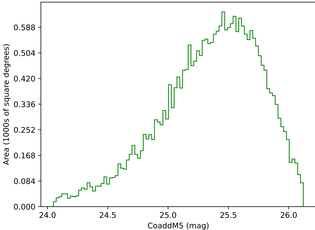
roll_pause_mjdp120_v3.4_10yrs Yr 3-4 g band: CoaddM5
