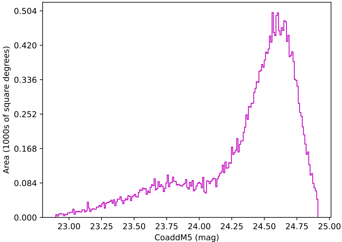
roll_pause_mjdp120_v3.4_10yrs Yr 1 z band: CoaddM5
