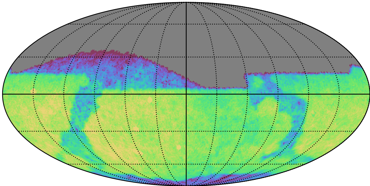
roll_pause_mjdp120_v3.4_10yrs Yr 1 i band: CoaddM5
