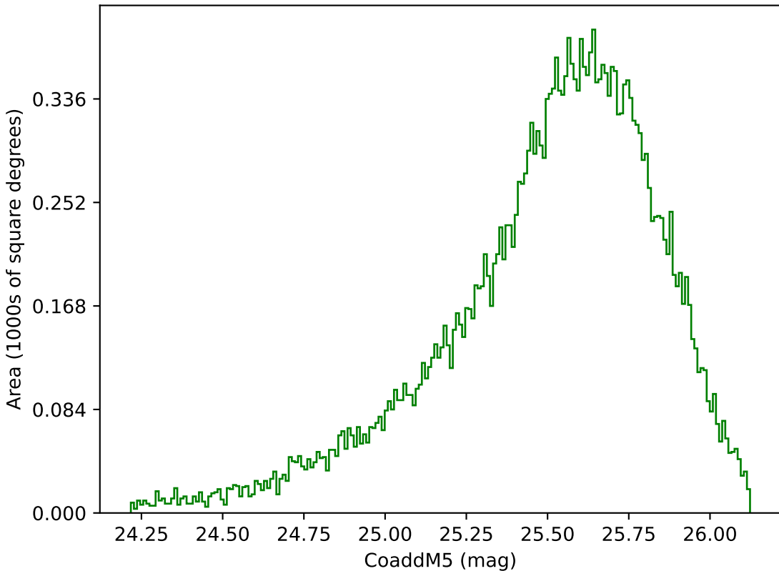
roll_pause_mjdp120_v3.4_10yrs Yr 1 g band: CoaddM5
