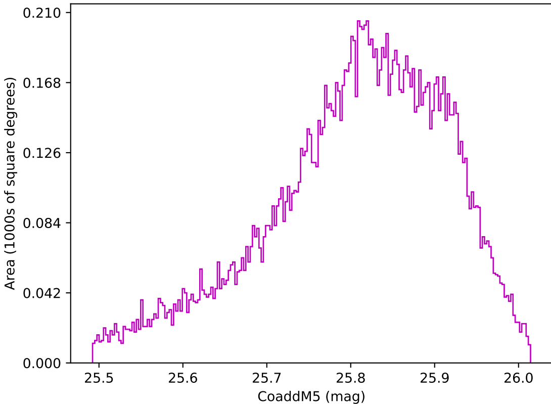
roll_pause_mjdp120_v3.4_10yrs WFD z band: CoaddM5
