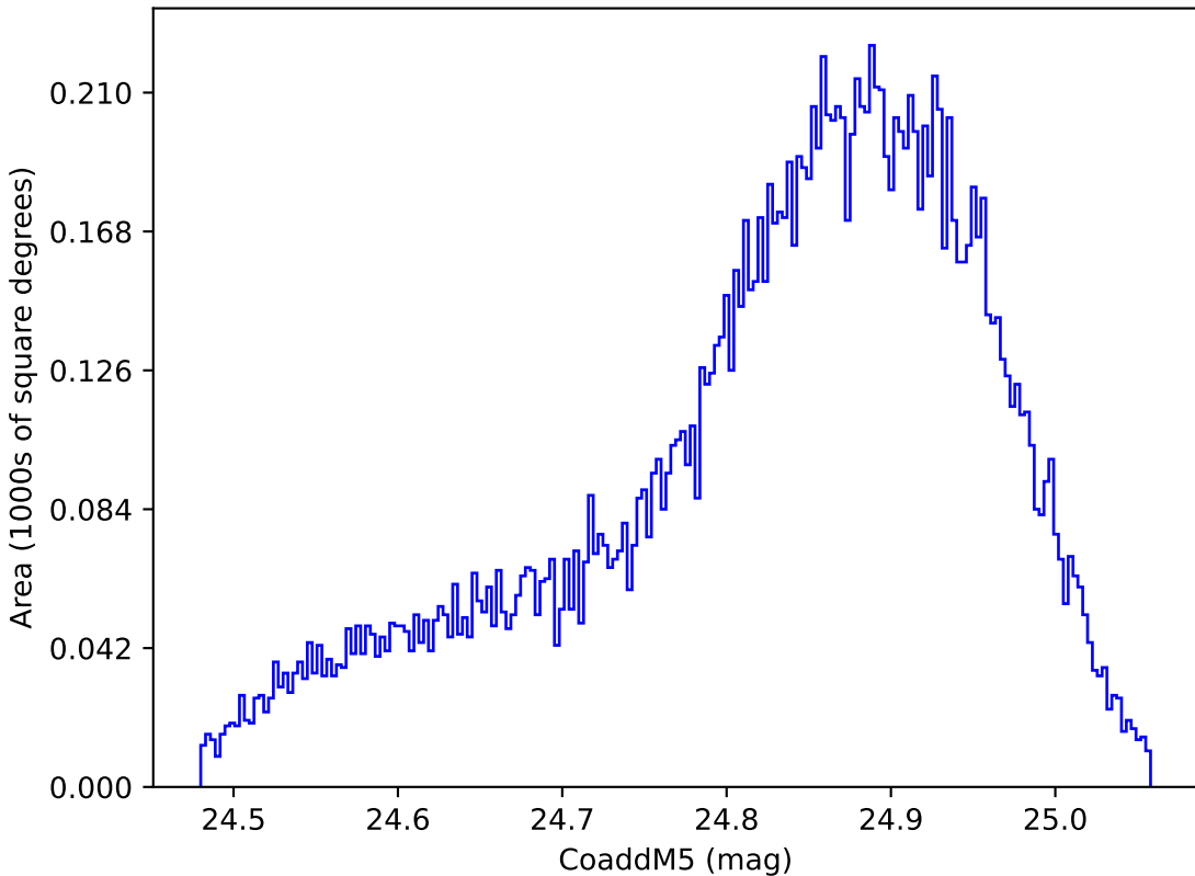
roll_pause_mjdp120_v3.4_10yrs WFD y band: CoaddM5
