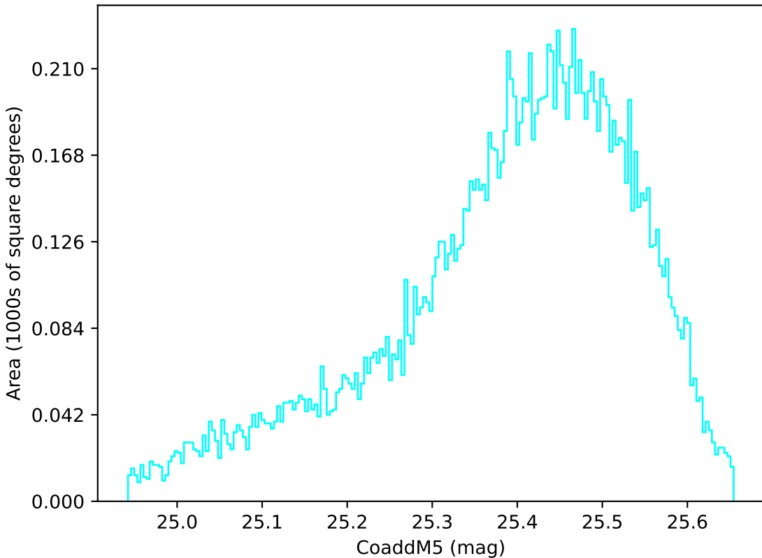
roll_pause_mjdp120_v3.4_10yrs WFD u band: CoaddM5
