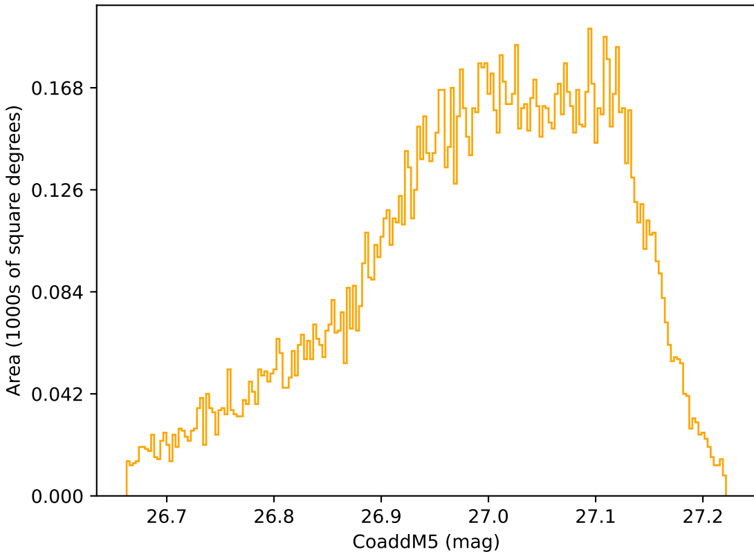
roll_pause_mjdp120_v3.4_10yrs WFD r band: CoaddM5
