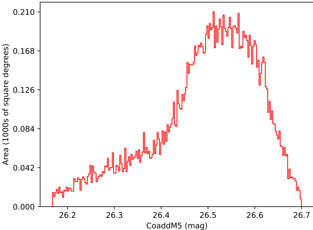
roll_pause_mjdp120_v3.4_10yrs WFD i band: CoaddM5
