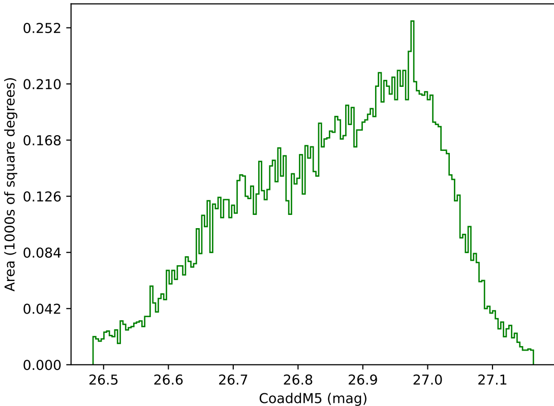
roll_pause_mjdp120_v3.4_10yrs WFD g band: CoaddM5
