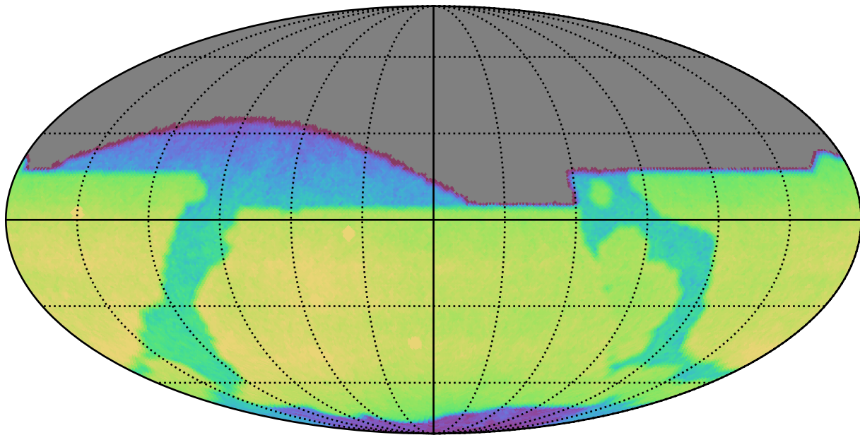
roll_pause_mjdp120_v3.4_10yrs All sky z band: CoaddM5
