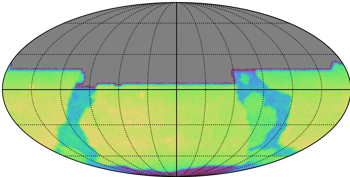
roll_pause_mjdp120_v3.4_10yrs All sky y band: CoaddM5
