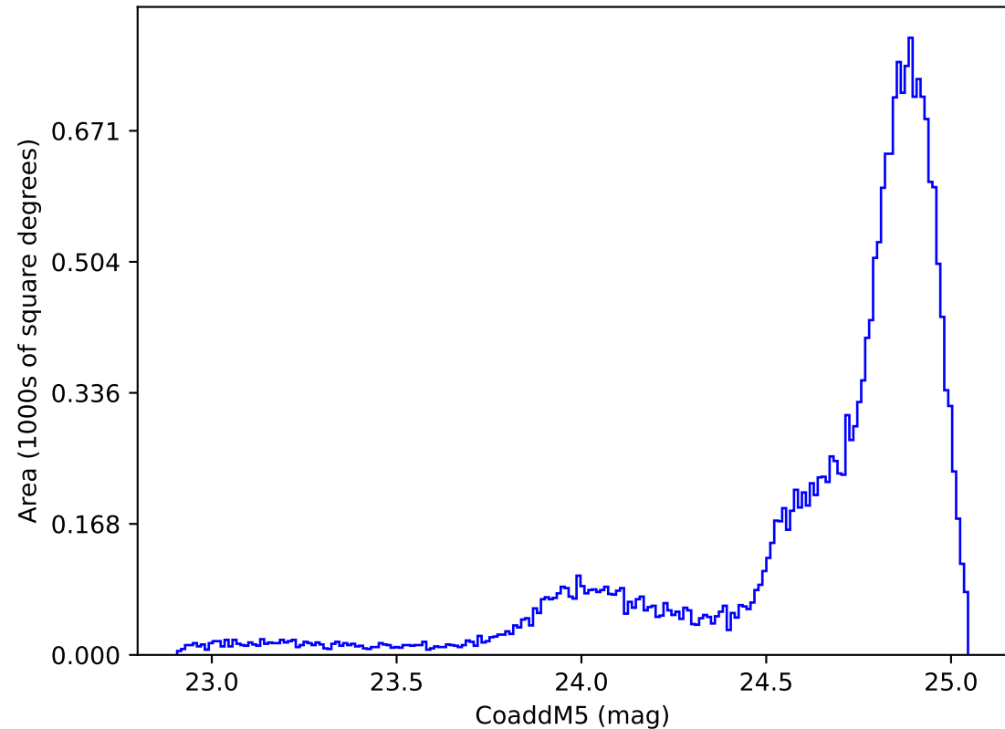
roll_pause_mjdp120_v3.4_10yrs All sky y band: CoaddM5
