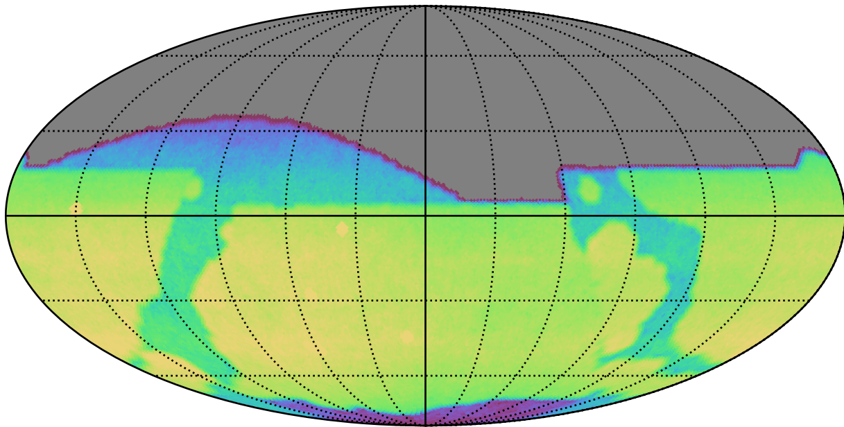
roll_pause_mjdp120_v3.4_10yrs All sky r band: CoaddM5
