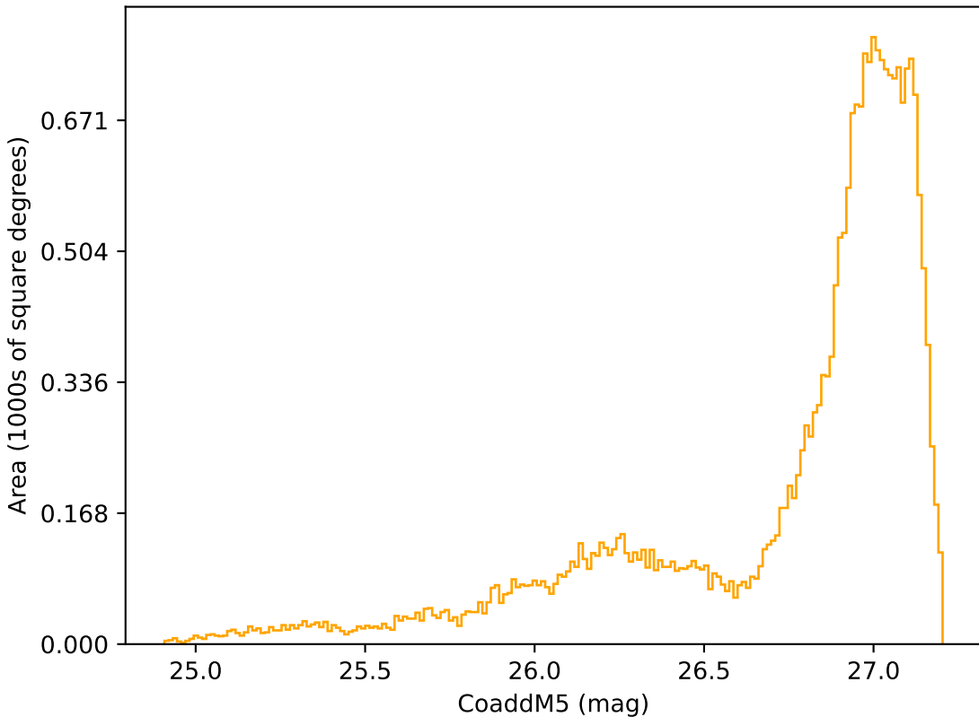
roll_pause_mjdp120_v3.4_10yrs All sky r band: CoaddM5
