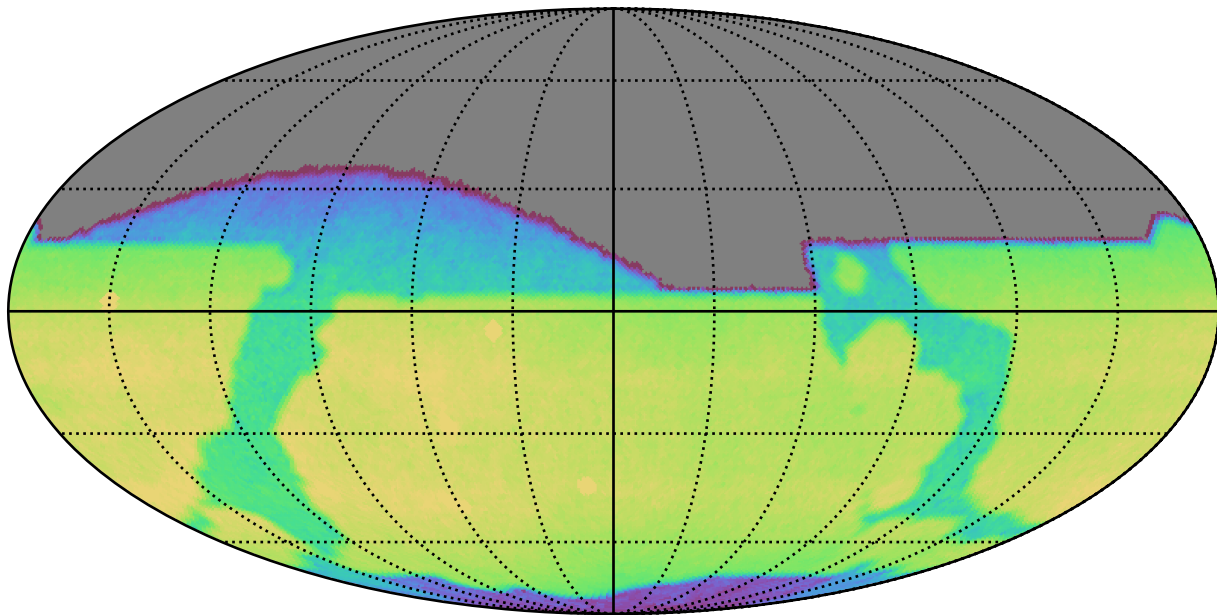
roll_pause_mjdp120_v3.4_10yrs All sky i band: CoaddM5
