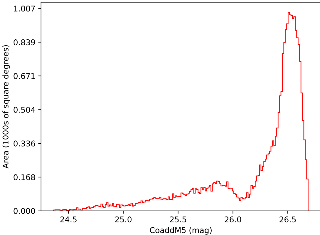
roll_pause_mjdp120_v3.4_10yrs All sky i band: CoaddM5
