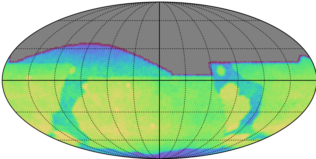
roll_pause_mjdp120_v3.4_10yrs All sky g band: CoaddM5
