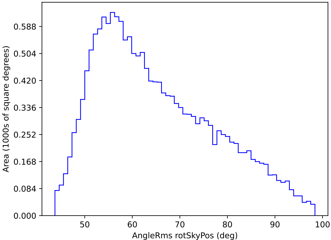
roll_pause_mjdp120_v3.4_10yrs WFD u band: AngleRms rotSkyPos
