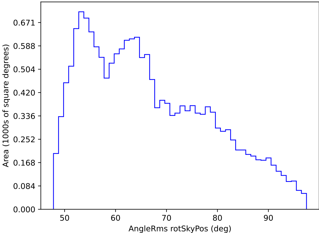
roll_pause_mjdp120_v3.4_10yrs WFD r band: AngleRms rotSkyPos
