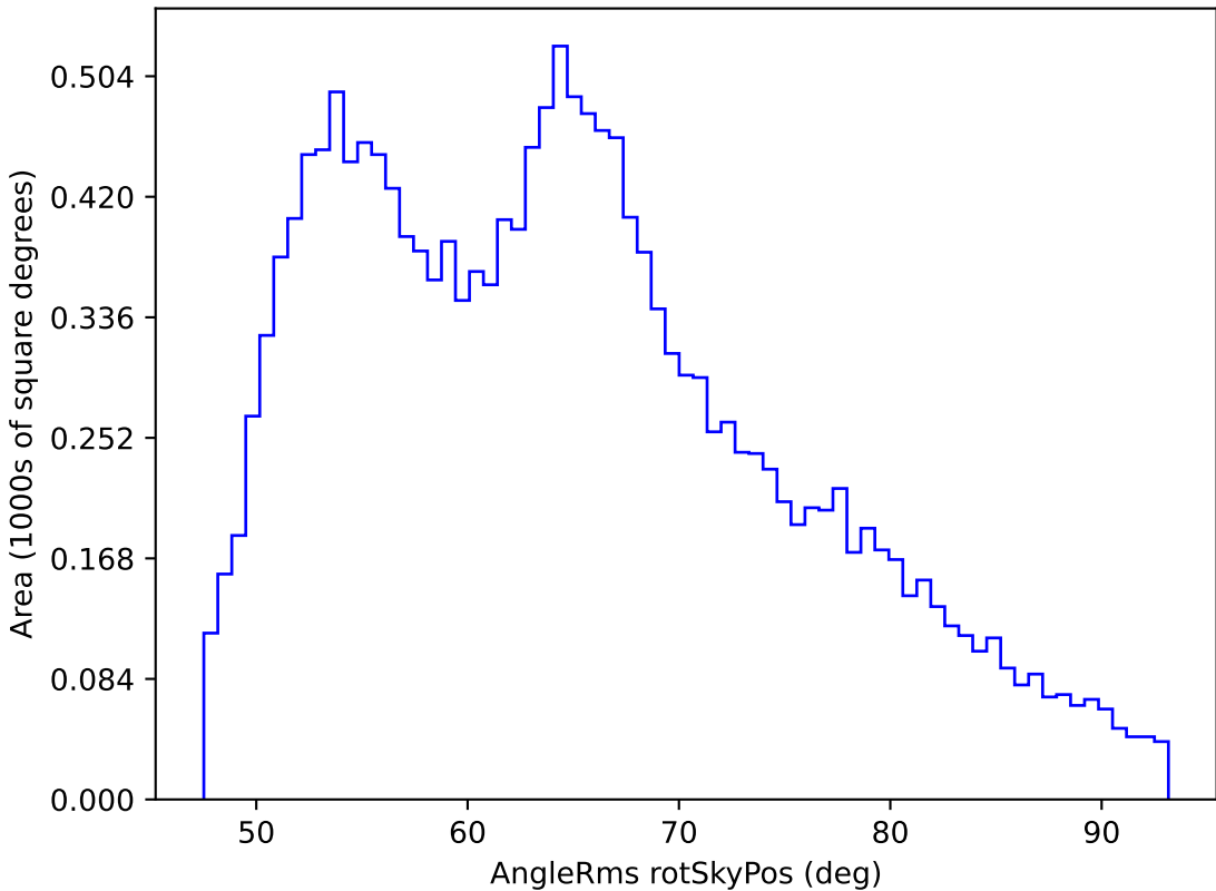
roll_pause_mjdp120_v3.4_10yrs WFD i band: AngleRms rotSkyPos
