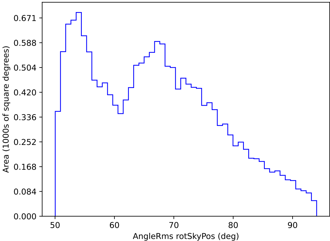
roll_pause_mjdp120_v3.4_10yrs WFD all bands: AngleRms rotSkyPos
