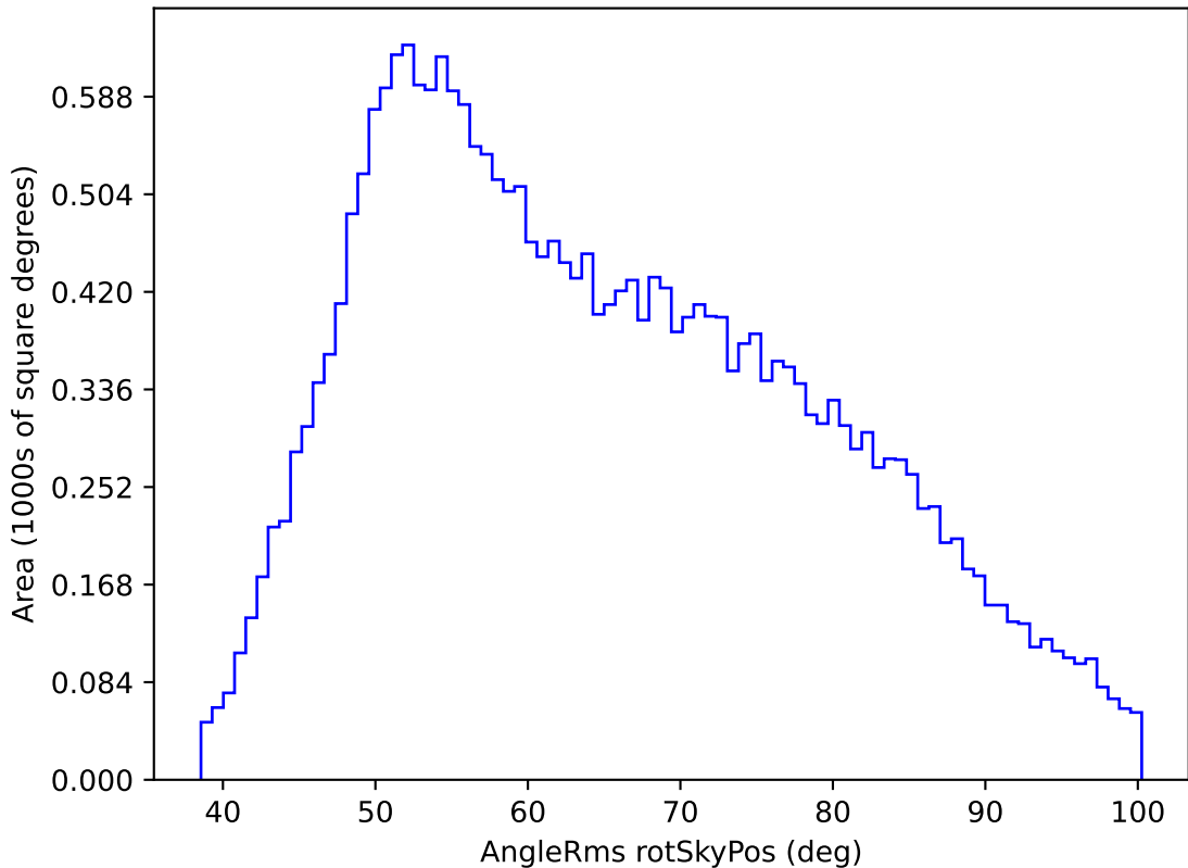
roll_pause_mjdp120_v3.4_10yrs All sky g band: AngleRms rotSkyPos
