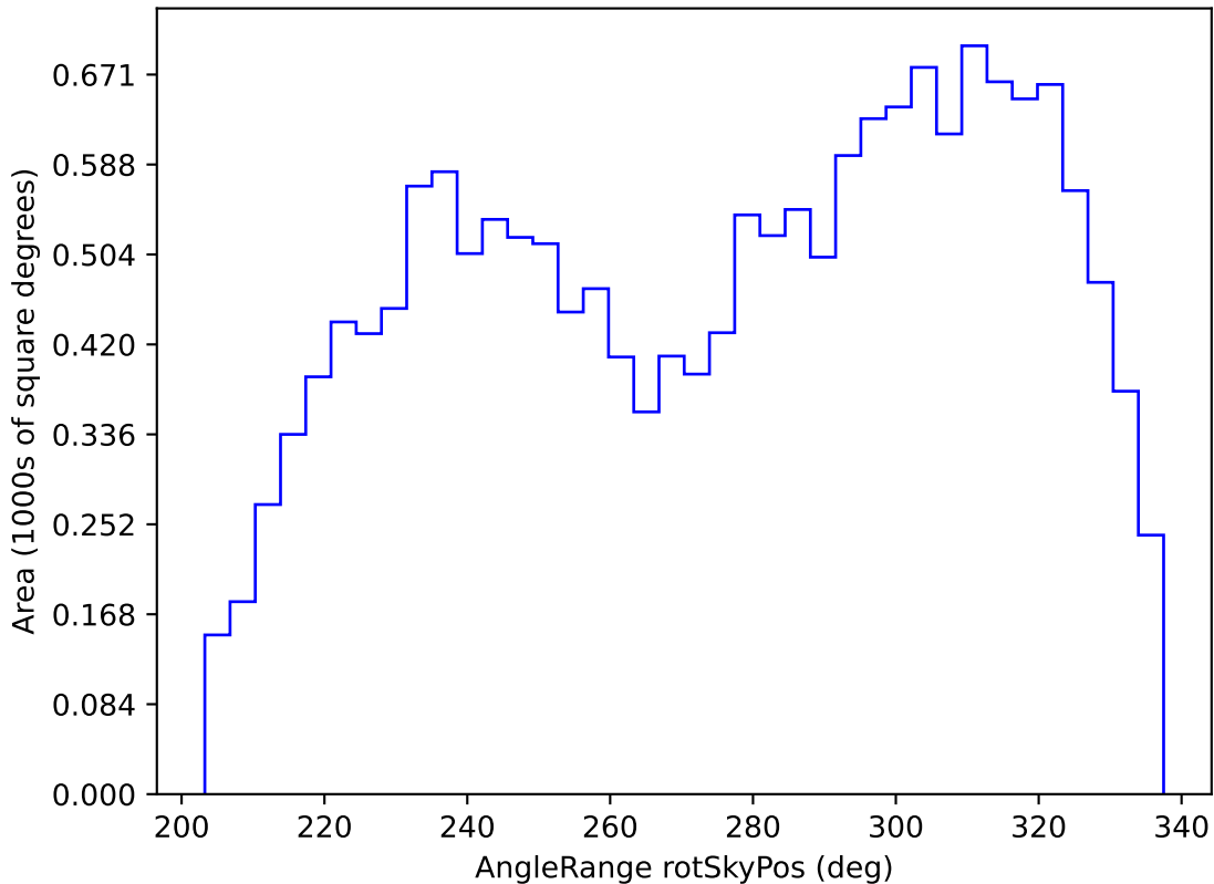
roll_pause_mjdp120_v3.4_10yrs WFD y band: AngleRange rotSkyPos
