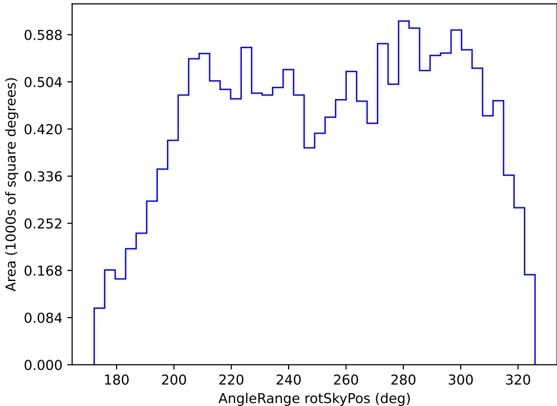
roll_pause_mjdp120_v3.4_10yrs WFD u band: AngleRange rotSkyPos
