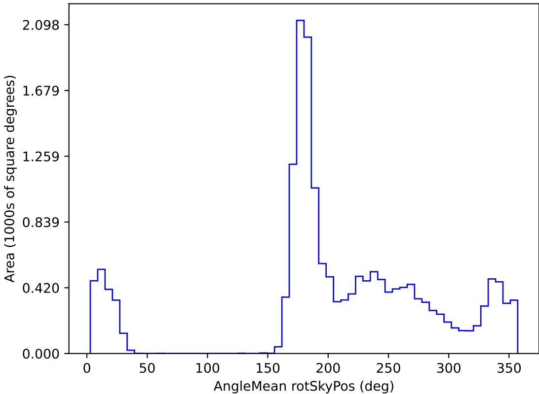
roll_pause_mjdp120_v3.4_10yrs WFD z band: AngleMean rotSkyPos
