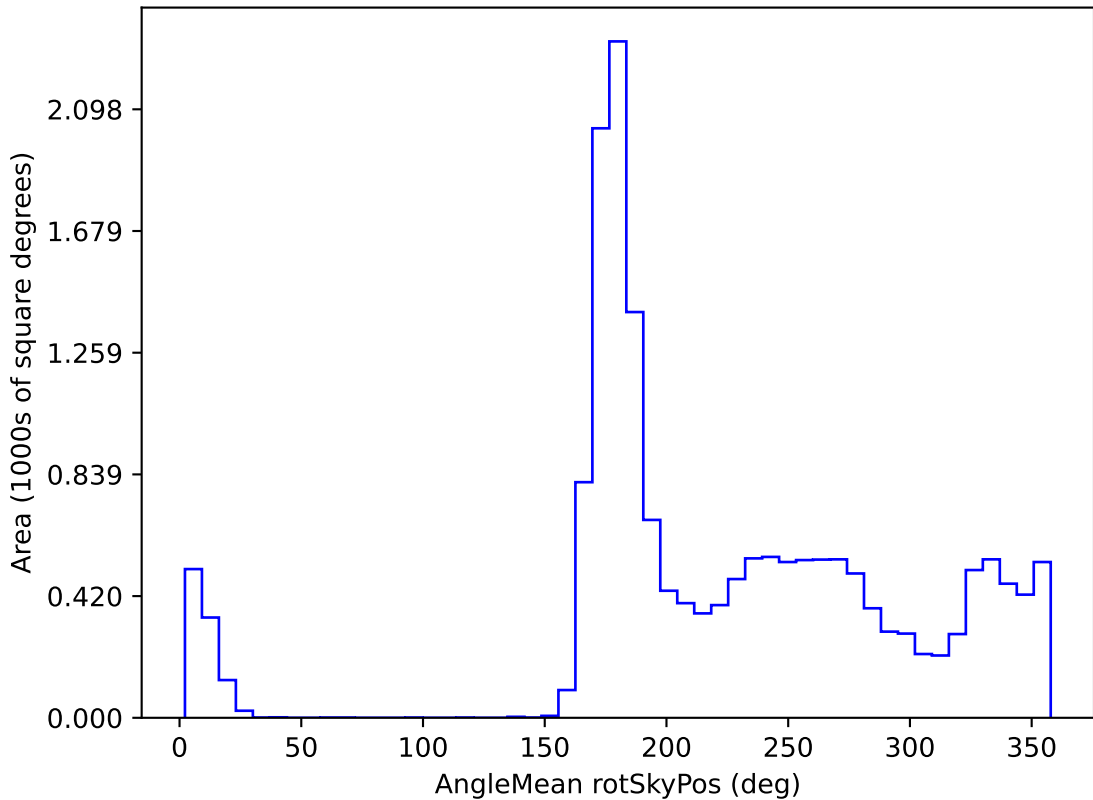
roll_pause_mjdp120_v3.4_10yrs WFD y band: AngleMean rotSkyPos
