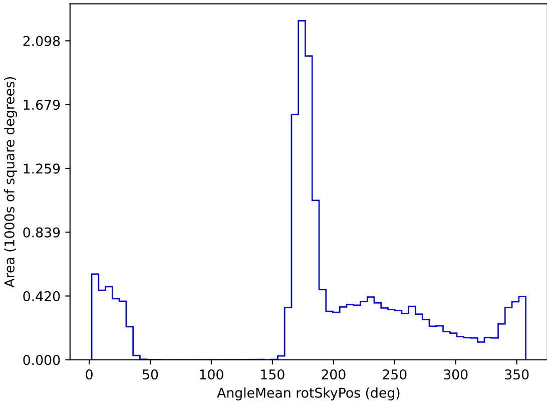
roll_pause_mjdp120_v3.4_10yrs WFD r band: AngleMean rotSkyPos
