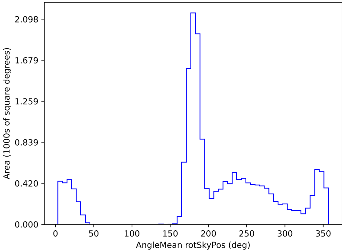
roll_pause_mjdp120_v3.4_10yrs WFD i band: AngleMean rotSkyPos
