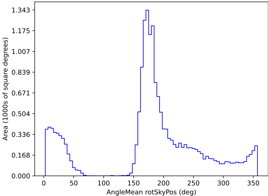
roll_pause_mjdp120_v3.4_10yrs WFD g band: AngleMean rotSkyPos
