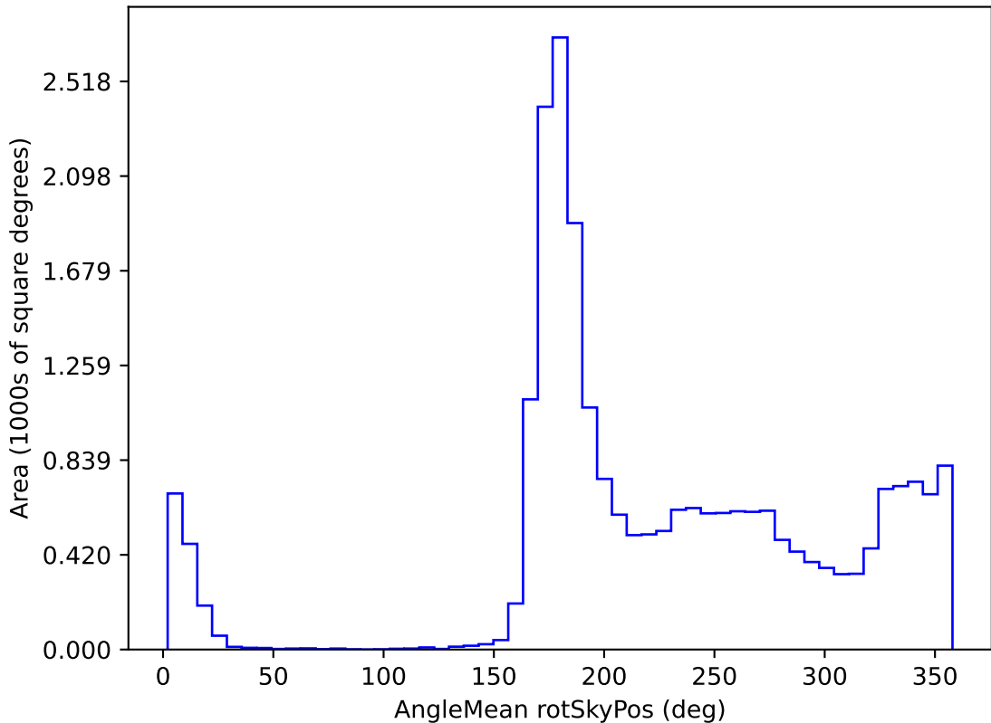
roll_pause_mjdp120_v3.4_10yrs All sky y band: AngleMean rotSkyPos
